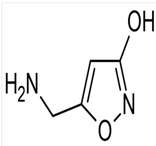
Chemical Structure - Muscimol, GABA A agonist (ab120094)
