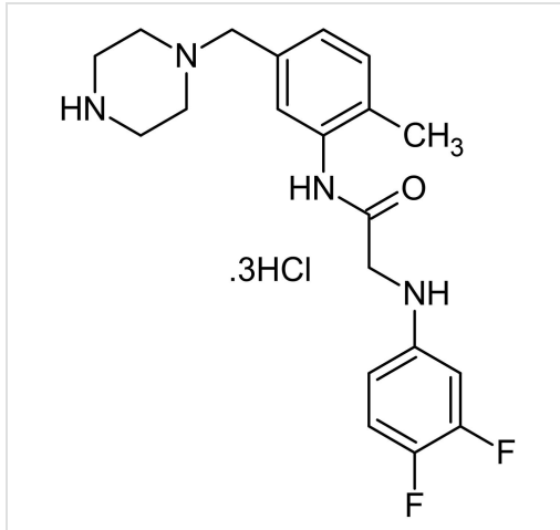
2D chemical structure image of ab120395, GW791343, P2X7 allosteric modulator
