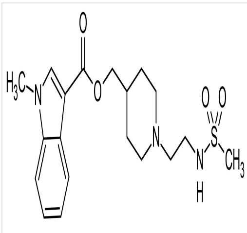
Chemical Structure - GR113808, selective 5-HT 4 antagonist (ab120544)
