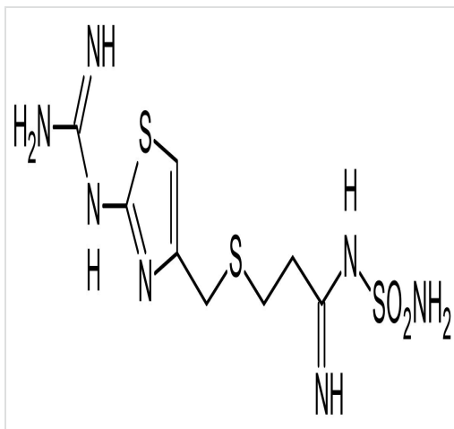
Chemical Structure - Famotidine, H 2 antagonist (ab120760)
