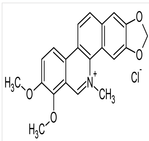
Chemical Structure - Chelerythrine chloride, Cell-permeable protein kinase C inhibitor (ab120600)
