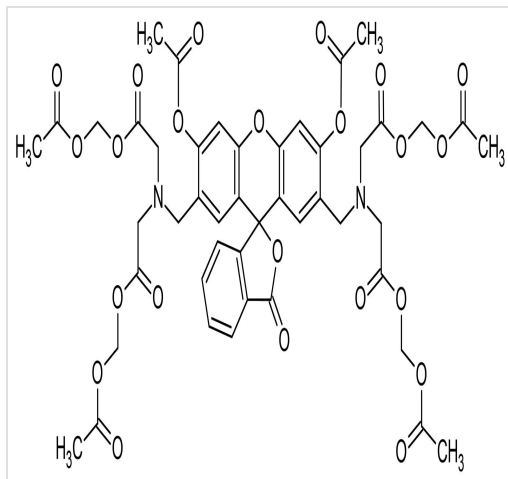
Chemical Structure - Calcein AM, fluorescent dye for cell viability (ab141420)
