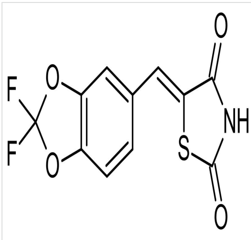
Chemical Structure - AS-604850, ATP-competitive PI3Kgamma inhibitor (ab120935)
