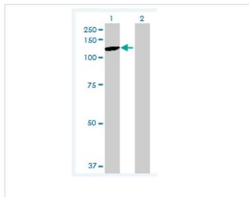
Western blot - PCDHGA10 antibody (ab68864)
