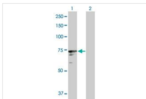
Western blot - ICK antibody (ab103817)
