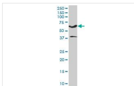
Western blot - ICK antibody (ab103817)
