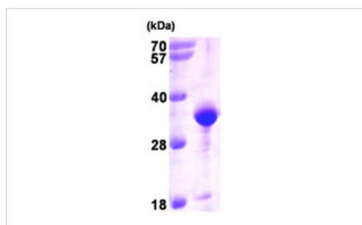
15% SDS-PAGE analysis of ab93462 (3µg).
