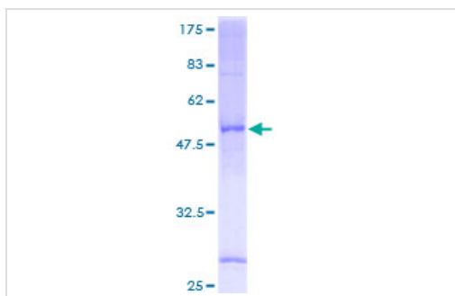
SDS-PAGE - SRD5A1 protein (Tagged) (ab116886)
