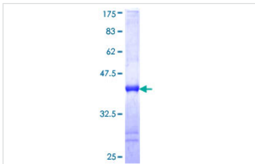
SDS-PAGE - RRAD protein (ab114746)
