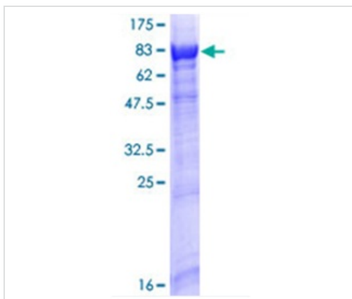
SDS-PAGE - RABGGTA protein (ab116789)
