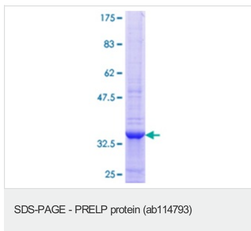
ab114793 on 12.5% SDS-PAGE Stained with Coomassie Blue.
