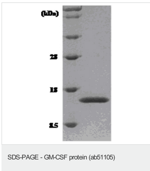
ab51105 in 14% SDS-PAGE
