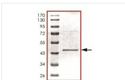
SDS-PAGE analysis of ab125548.
