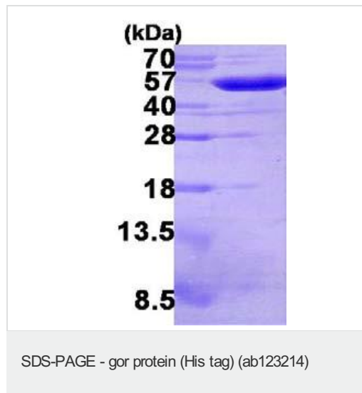
15% SDS-PAGE showing ab123214 (3 µg) at approximately 51.2 kDa.
