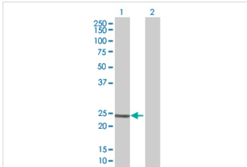
Western blot - Anti-RAB37 antibody (ab67267)
