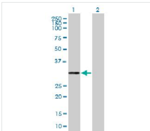
Western blot - PR3 antibody (ab88097)
