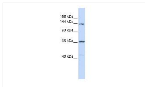
Western blot - Anti-PCDH12 antibody (ab82885)
