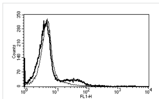
Flow Cytometry - Anti-NCAM1 antibody [B-A19] (ab27299)
